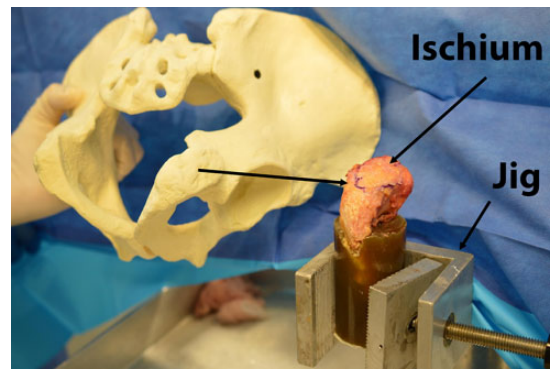
Figure 1. Cadaveric dissection demonstrating the testing setup for hamstring load to failure on a right ischium. A Sawbones model of the pelvis is included to facilitate 3-dimensional understanding of the position of the bone.
